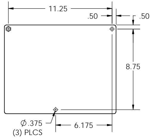
MOUNTING PATTERN
